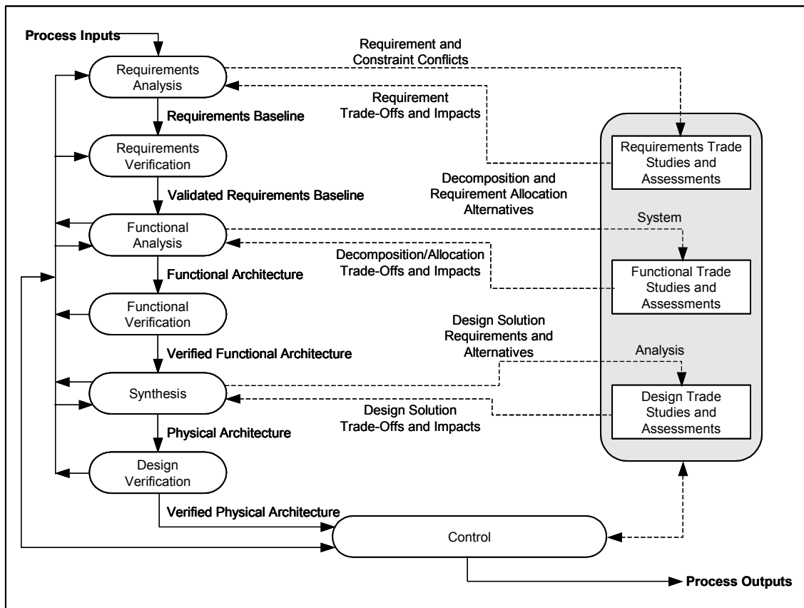
Figure 3-6. IEEE Std 1220-1998 Systems Engineering Process
