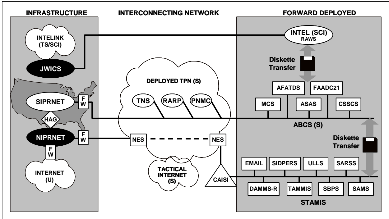
Figure 9-4. Near-Term Architecture [11]
