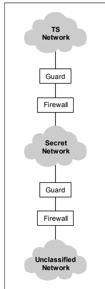
Figure 6.3-3. Cascading Protection
