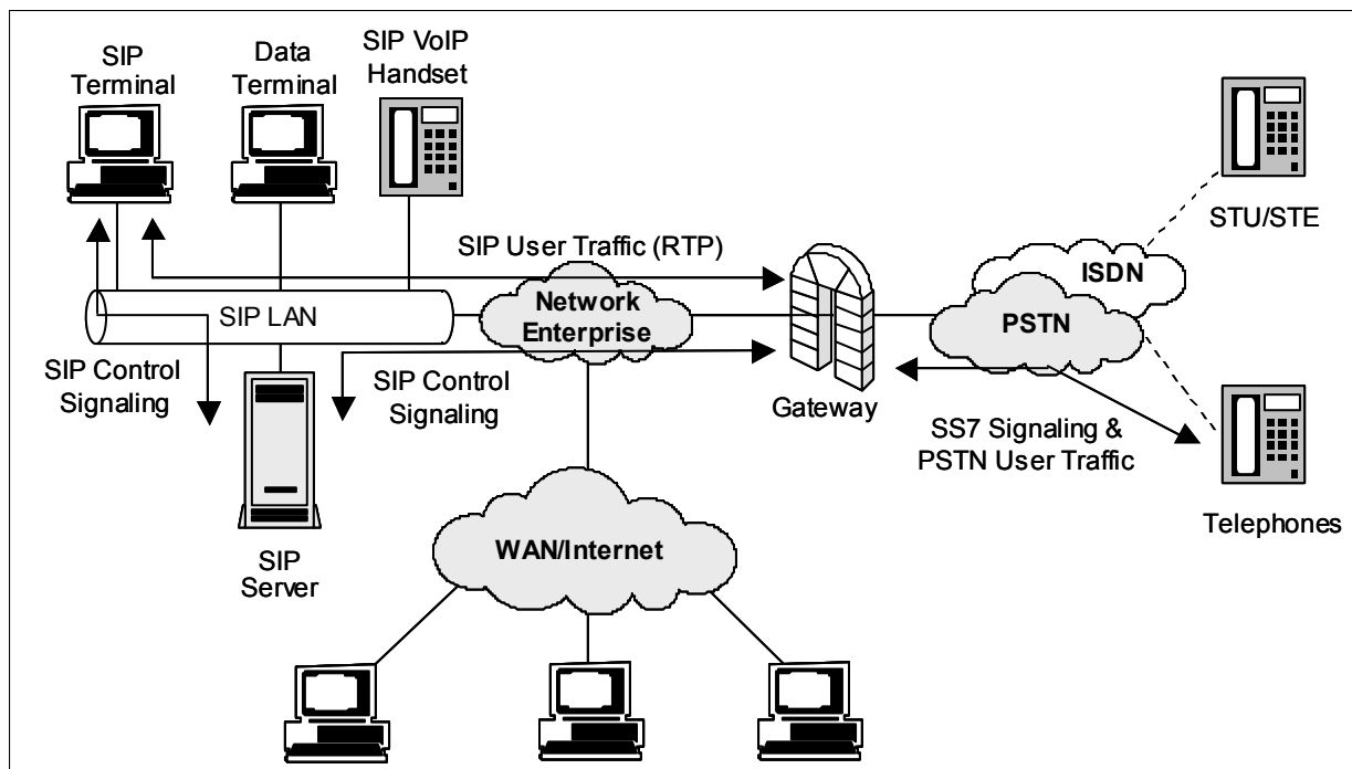
Figure 5.4-1. SIP Network
