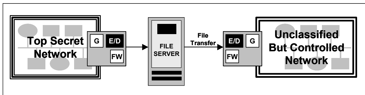
Figure 6.3-4. File Transfers
