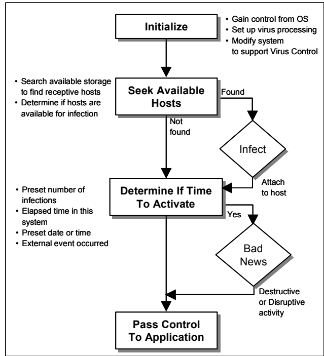
Figure 6.6-3. Virus Execution
